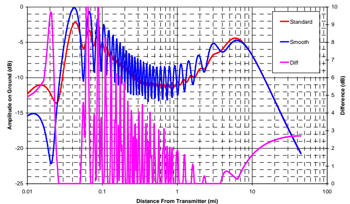
Figure 2: Relative Signal Strength on Smooth Earth
