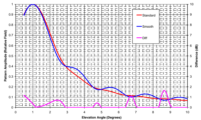
Figure 1: Standard and Smooth Elevation Patterns
